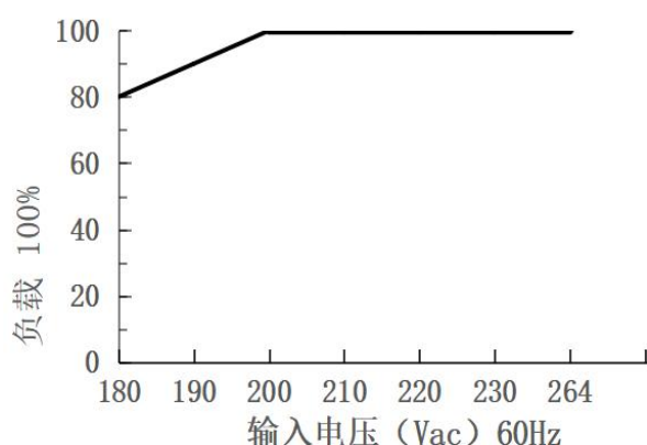
■ 降额曲线 Derating Curve
