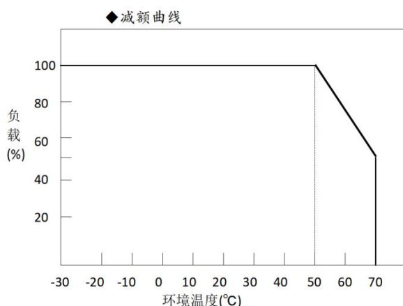
■ 降额曲线 Derating Curve
