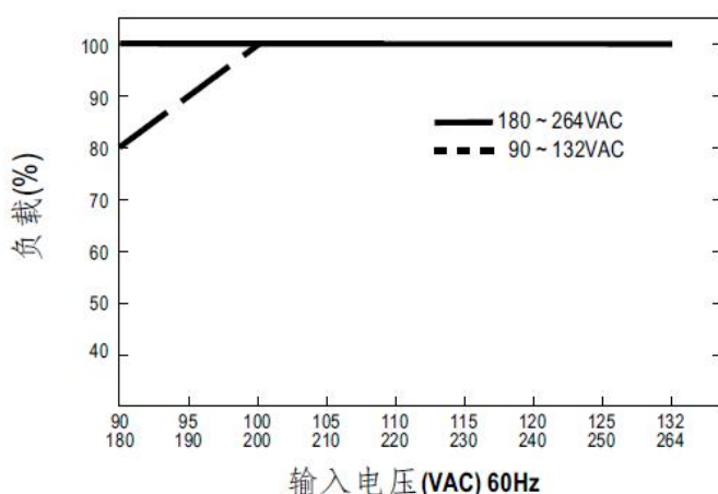
■ 降额曲线 Derating Curve
